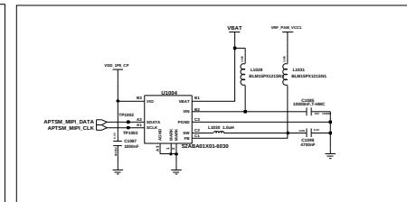
APT MODULATOR
